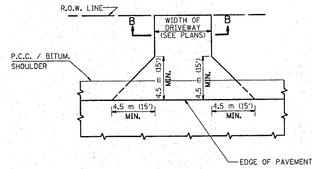
ADJACENT TO P.C.C. / BITUMINOUS SHOULDER
